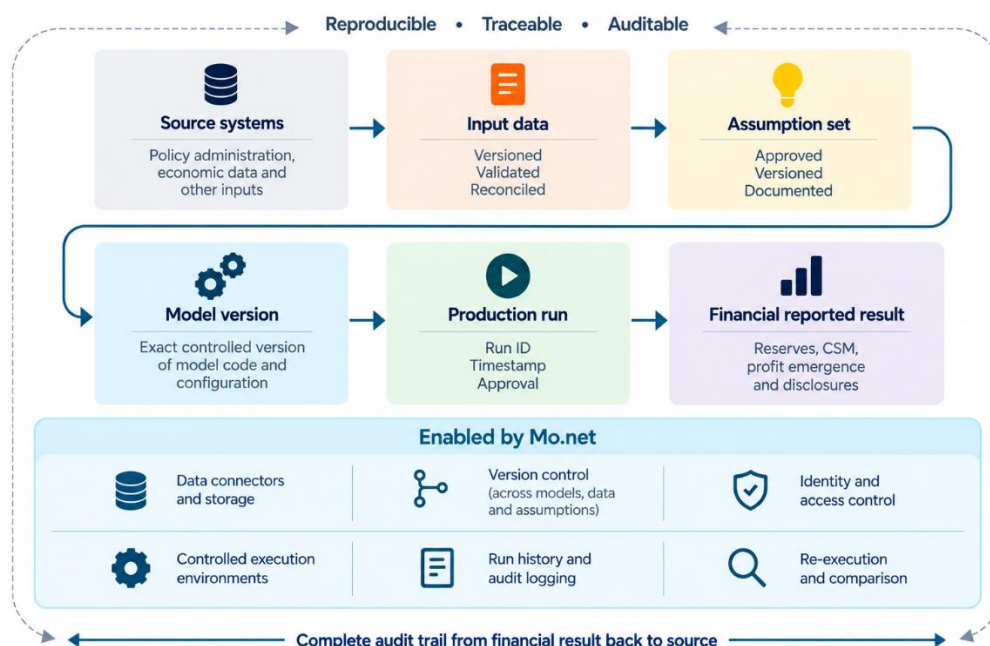
Figure 3 - End-to-End Traceability and Reproducibility
